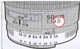
② CPU Nikon lens other than G-type
